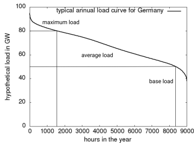
Fig. 1. – Typical annual load curve that displays how much load is required in a given grid (y-axis) for how many hours in a year (x-axis). Typical recent annual load curves for germany can be found for example in [1]. Figure data based on [2].
