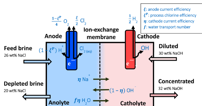
Fig. 11. – Schematic overview of a membrane-based chlorine alkaline electrolyser. Figure adapted with permission from [46].
