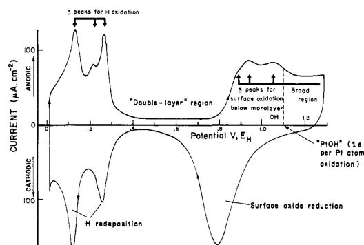
Fig. 7. – Cyclic voltammogram: Potentiodynamic current-potential profile for a polycrystalline platinum electrode aqueous sulfuric acid. Figure adapted with permission from [35].
