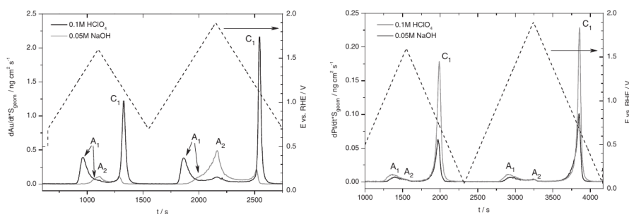
Fig. 19. – By coupling a mass spectrometer to an electrochemical flow cell, the group of Mayrhofer was able to study noble metal corrosion in detail. The dashed lines indicate the applied potential while solid lines quantify dissolved noble metal ions. [79] The investigation of gold corrosion (left) and platinum corrosion (right) show that for both cases no continuous corrosion occurs, but noticeable amounts of noble metal are dissolved while reducing the oxide formed at higher potentials. Figure reproduced from [80] under Creative Commons licence (Attribution-NonCommercial-NoDerivatives 4.0 International CC BY-NC-ND 4.0).
