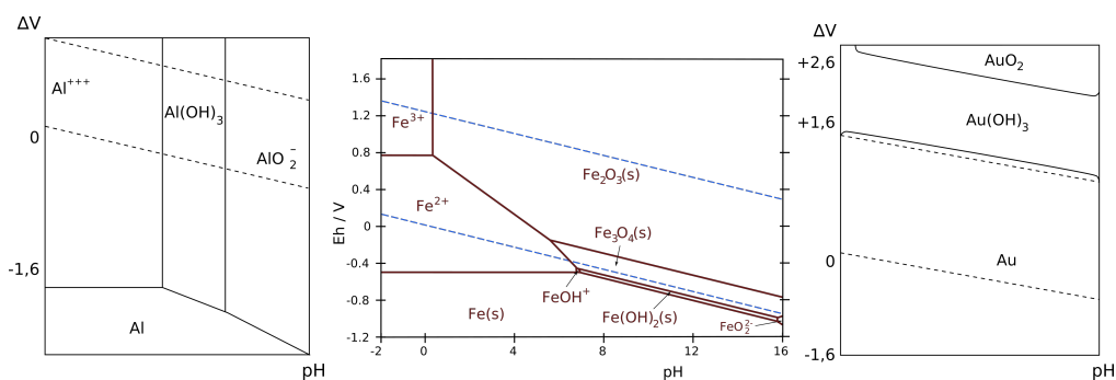
Fig. 6. – Pourbaix diagrams for aluminium, iron and gold. Dashed lines denote stability window of water. (Source: Wikimedia commons.wikimedia.org/wiki/File:Fe-pourbaix-diagram.svg, commons.wikimedia.org/wiki/File:D-pourbaix-Al.svg, commons.wikimedia.org/wiki/File:Pourbaix-Au.svg under Creative Commons Attribution-Share Alike 3.0 Unported license.)
