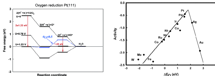
Fig. 15. – Nørskov and coworkers discuss the origin of the overpotential for the ORR in detail. Left: Computed reaction path depending on the applied potential. Right: Volcano plot for the ORR, for which the oxygen adsorption strength is plotted against the activity of a catalyst material. Figure reproduced with permission from [59].
