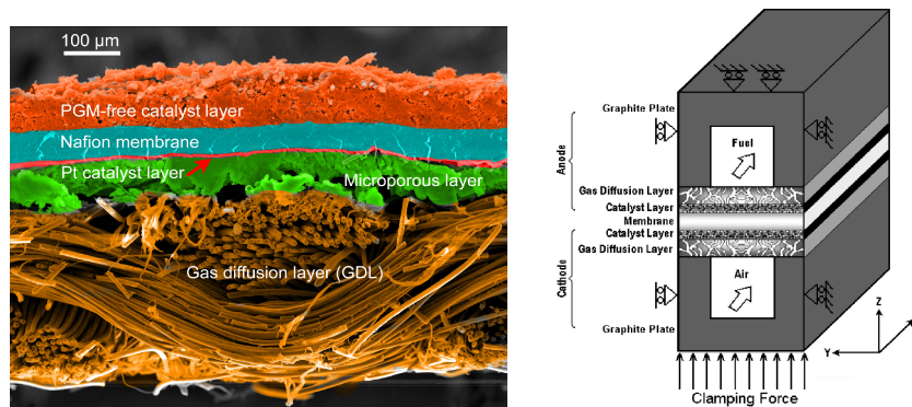
Fig. 14. – Left: Scanning Electron Microscopy (SEM) micrograph of a PEMFC MEA (see also [55]). Source: Wikimedia ( commons.wikimedia.org/wiki/File:SEM_micrograph_of_an_MEA_cross_section.jpg ) by Xi Yin under Creative Commons Attribution-Share Alike 4.0 International license. Right: Schematic view of the corresponding cell. With permission from [56]. Note that in practice, several extended cells of this type will be stacked to obtain the actual fuel cell.
