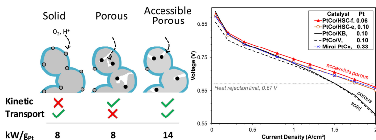
Fig. 17. – Yarlagadda et al. report on how different types for porestructures in carbon material influence catalyst activity. Black cycles denote active, grey cycles denote less active nanoparticles, blue denotes adsorption of ionomer on the support material. The panel on the right shows how increased activity is obtained when accessible pores are available. Figure reproduced with permission from [70].
