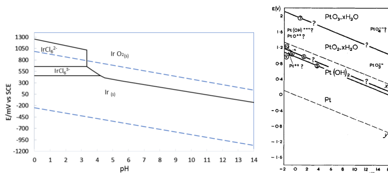
Fig. 18. – Left: Pourbaix diagram from iridium (in HCl), dashed lines denote the stability window of water. Right: Pourbaix diagram for platinum. Reproduced from [74] under Creative Commons Attribution 4.0 International License. Reproduced from [75] under Creative Commons Attribution-NonCommercial-NoDerivatives 4.0 International License.
