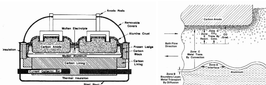
Fig. 12. – Typical cell setup for the Hall-Héroult process (left) and closeup schematics of the interface regions. Figure adapted with permission from [47].
