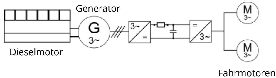
AC-AC
